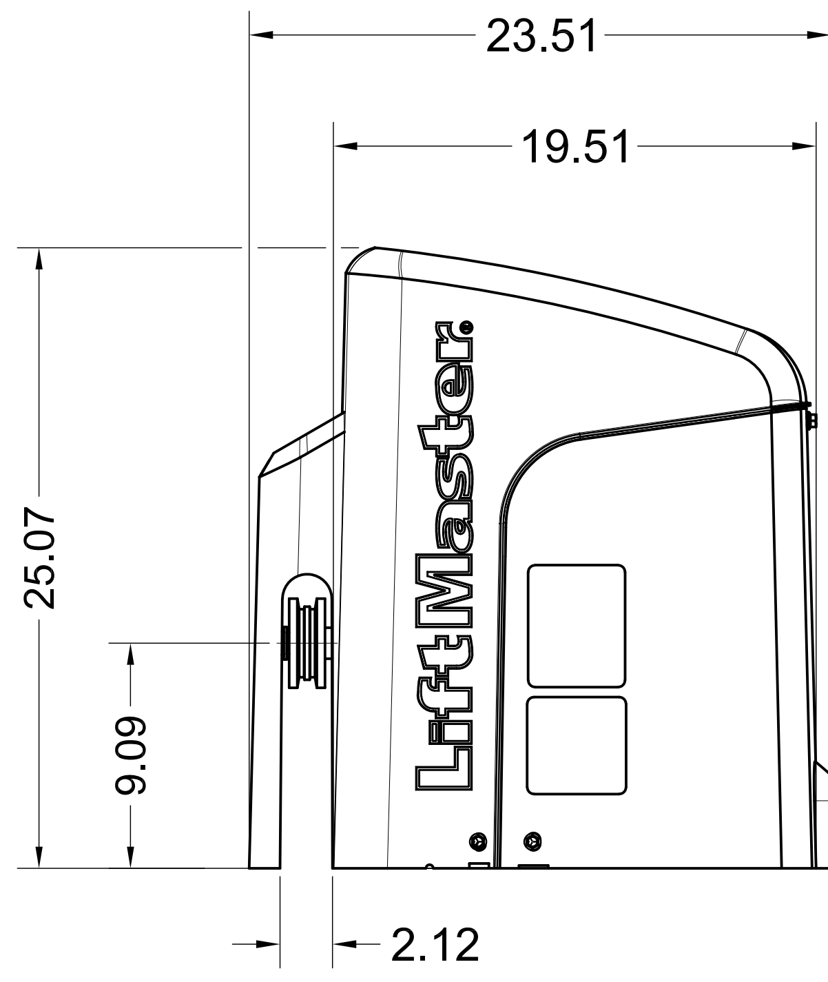
LEFT VIEW
